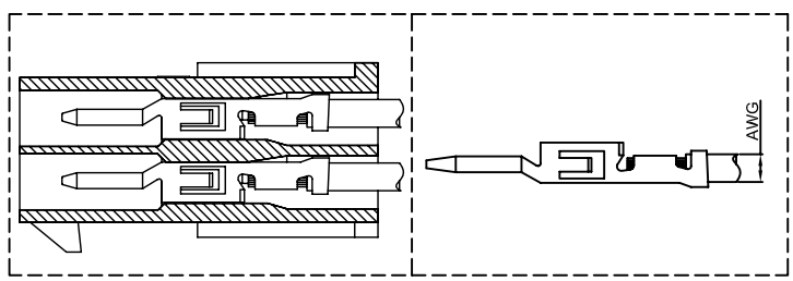
TERMINAL ASSEMBLY DRAWING
