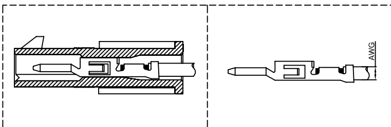
TERMINAL ASSEMBLY DRAWING
