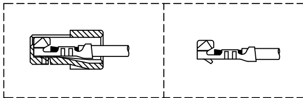
TERMINAL ASSEMBLY DRAWING
