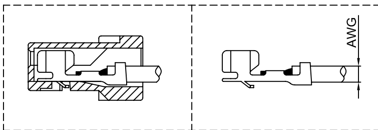
TERMINAL ASSEMBLY DRAWING
